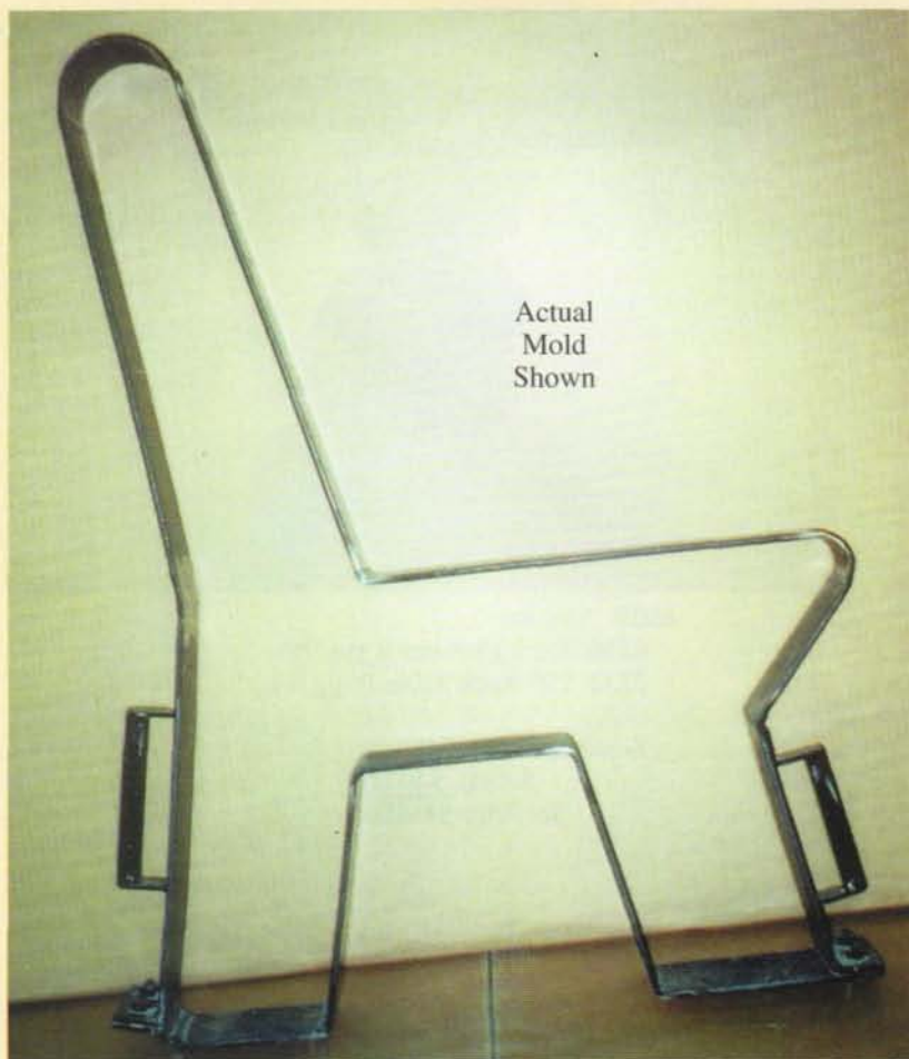
558 Park Bench Leg Mold 35"H x 4" thick Use with 2"x4" wood seat and back. Predrilled for Anchor Placement. Steel
